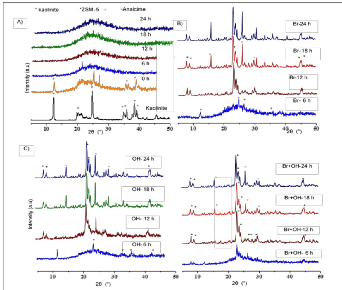
27 Fig. 1 XRD patterns of samples A) kaolin and without template, B) TPABr (Br), C) TPAOH (OH), and D) TPAOH + TPABr (Br + OH) template
