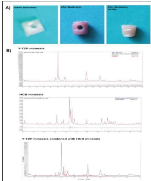
Figure 1. Distortion of Y-TZPSs. A) Y-TZP had grooves and holes in the rod section with size (Ø = 2.9mm, P = 3mm). B) mineral analysis with XRD examination. The peak on the graph of material analysis with XRD examination of Y-TZP minerals, HCB minerals, and Y-TZP minerals combined with HCB minerals
