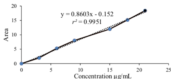
Figure 3. Linearity graph analytical validation pada 254 nm.
